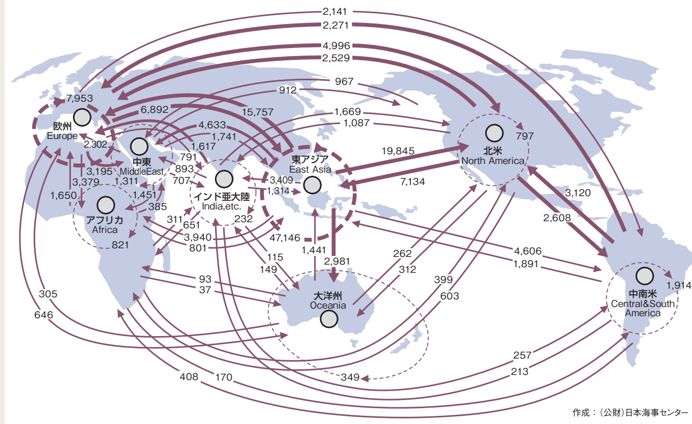
World Container Estimated Movement in 2021
